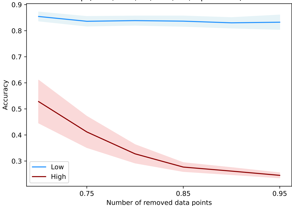
DataAttrOpt(5000, 0.03, 15, best, +b, alpha=best) - nomao
